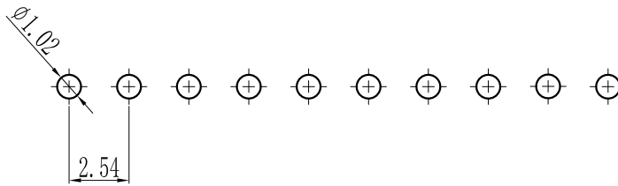
PCB LAYOUT
