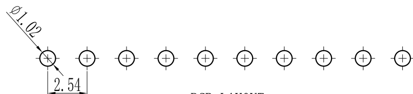
PCB LAYOUT
