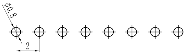
PCB LAYOUT
