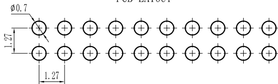
PCB LAYOUT
