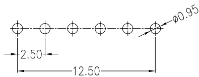
Board Layout
