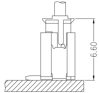
Assembly Layout
